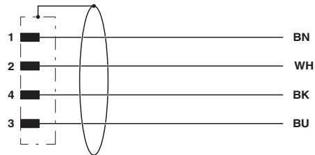
Contact assignment of M8 plugs/sockets
